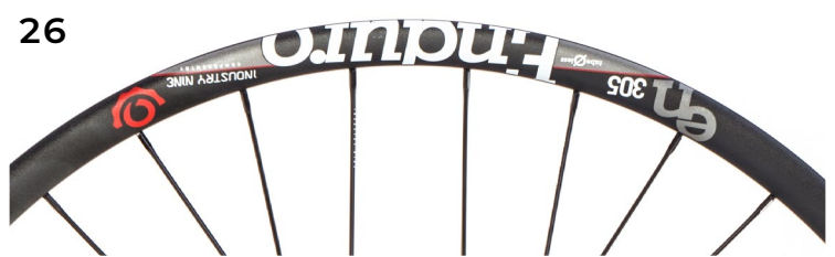
2015-16 | Enduro 305 V1 Alloy | Rim + Graphic Change 30.5mm IW | 26" ERD 532 | 27.5" ERD 560 | 29" ERD 597 32H 26" DS 266mm | Non-DS 268mm 32H 27.5" DS 278mm | Non-DS 280mm 32H 29" DS 297mm | Non-DS 299mm
